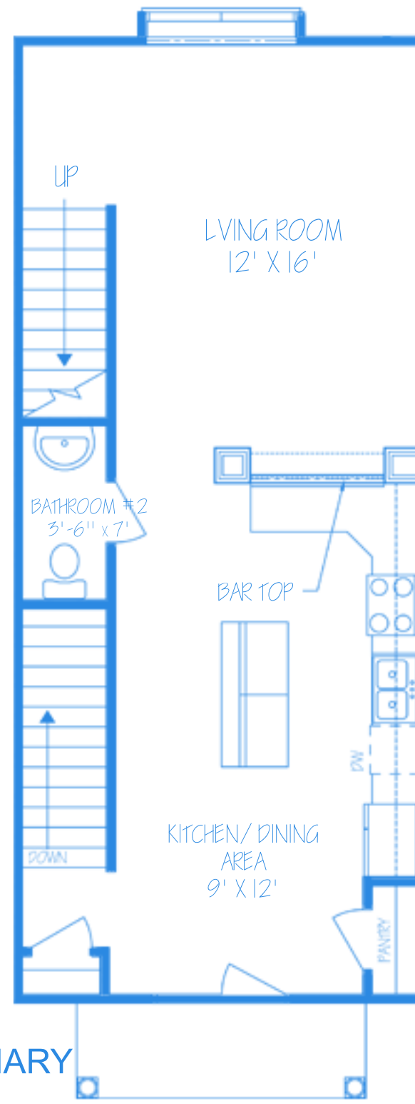
Monticello Second Floor Plan
